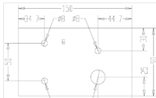
Abb. 2: Rückwand SchlüsselDepot 5mm
