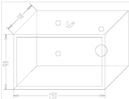
Abb. 1: Korpus SchlüsselDepot 5mm
